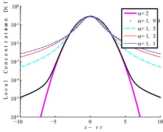
FIG. 1: The conservative component u(x, t) with a delta initial condition for various values of \alpha for K = 0.1 and at t = 1/D_\alpha .
