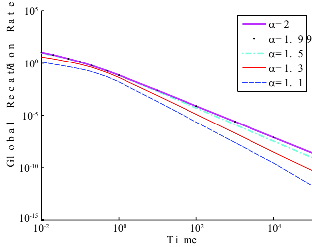
FIG. 4: The global reaction rate R against time for various values of \alpha and K = 0.1 .
