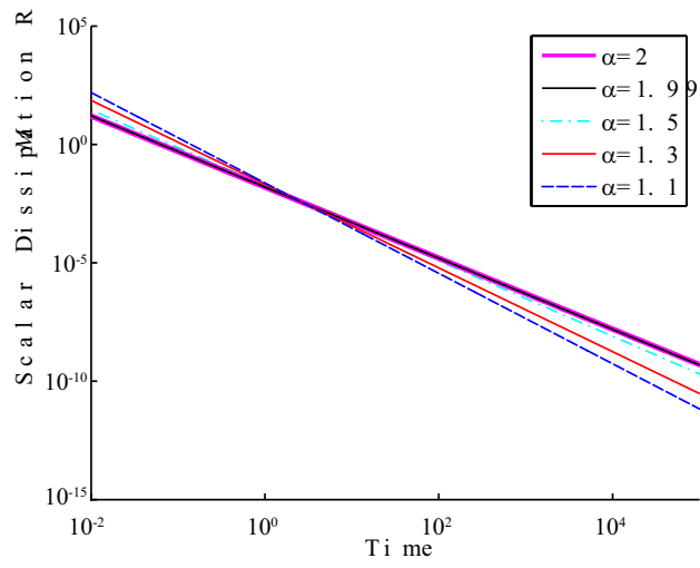
FIG. 3: The scalar dissipation M against time for various values of \alpha .
