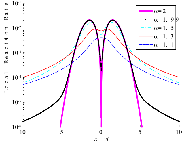
FIG. 2: Local reaction rate r with a delta initial condition for u for various values of \alpha at t = 1/D_\alpha and K = 0.1 .
